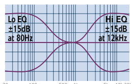
LF and HF EQ curves
