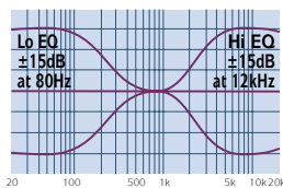
LF and HF EQ curves
