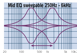
Swept Mid EQ curve
